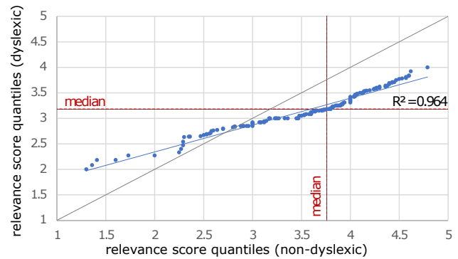
Figure 2: Q-Q plot comparing the relevance score quantiles of both groups. (Dyslexic: vertical, non-dyslexic: horizontal)
